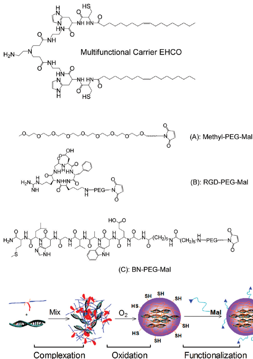
Figure 1. Chemical structures of EHCO, thiol reactive PEG and peptide PEG conjugates, and the scheme of preparation of ligand-directed siRNA delivery system.
